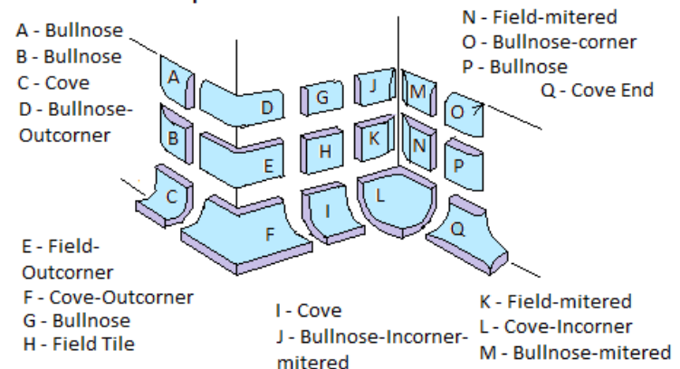
Exploded View - Trim Tiles
